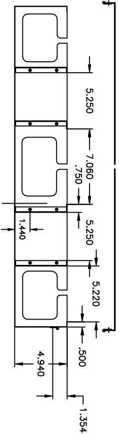
SECTION C-C
